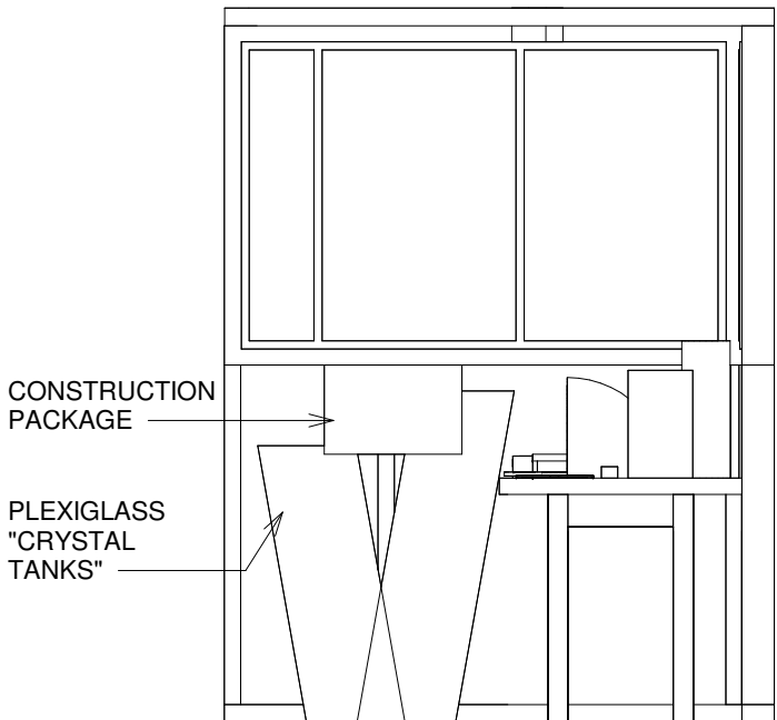
2 East 1/2" = 1'-0"
