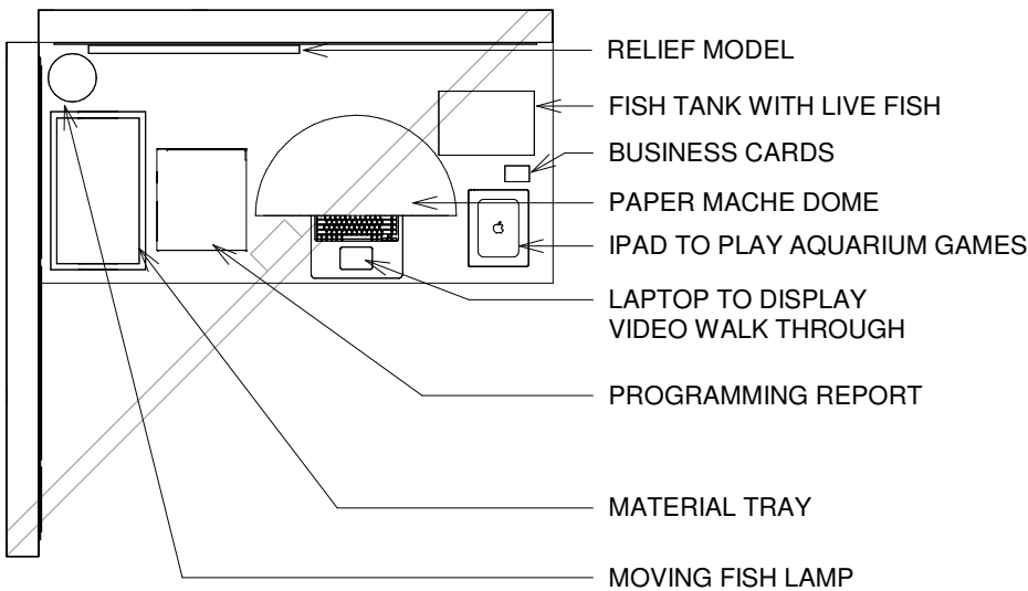
1 Level 1 1/2" = 1'-0"
